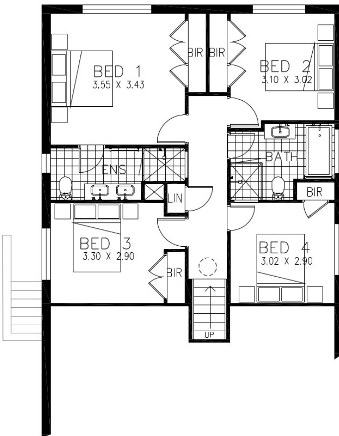
UPPER LEVEL
