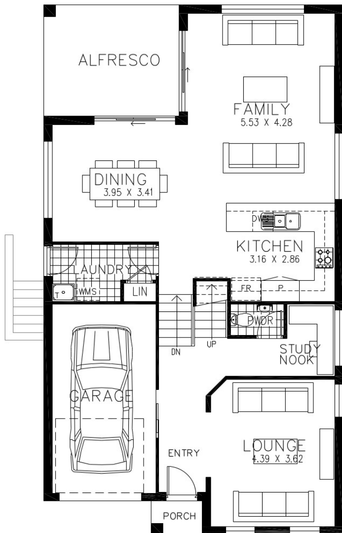
ENTRY LEVEL
